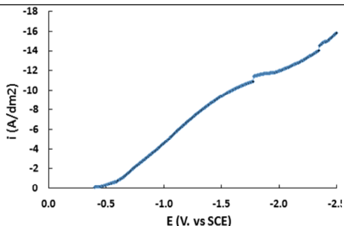
Figure 1. Cathodic polarization curve of studying solution.
